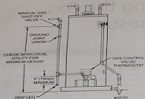
Fig. 1. Gas Piping.
