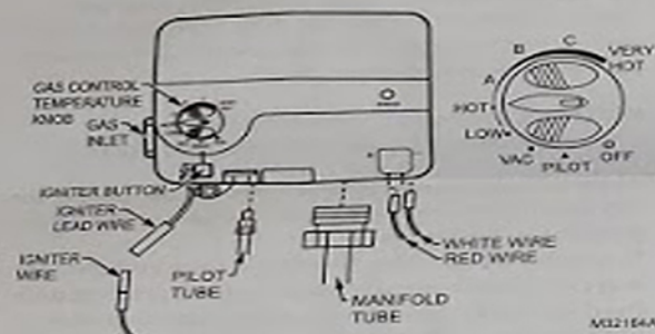
Fig. 2. Gas Control Valve/Thermostat
